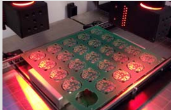
Speedline stencil printers handle boards for SMT 01005 and 0201.
